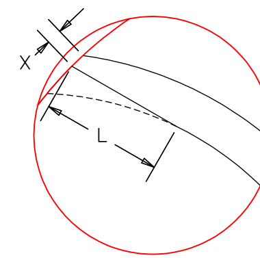
DETAIL Z VANE UNDERFILING
