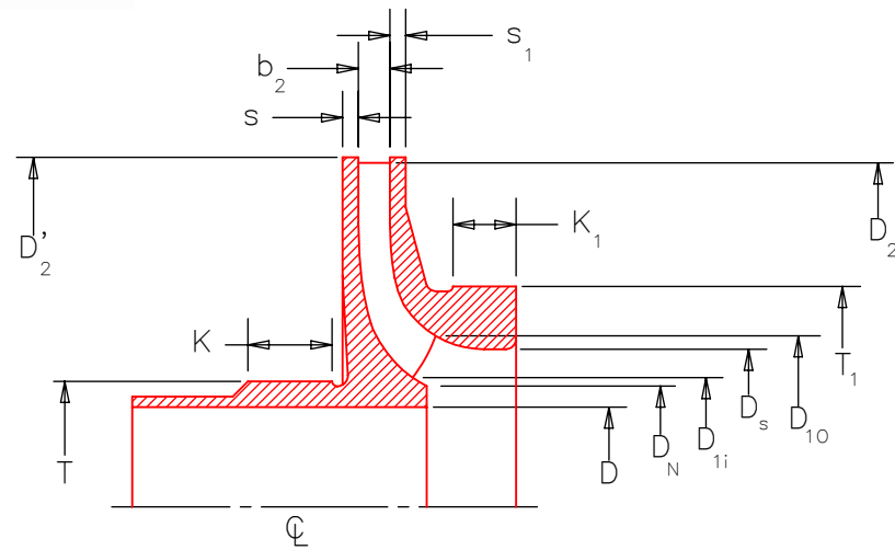
LOW SPECIFIC SPEED
