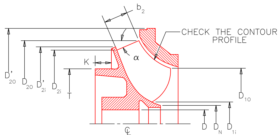
SEMI-OPEN IMPELLER
